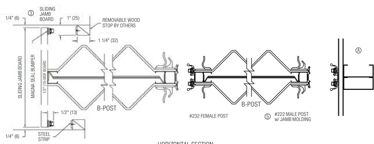
HORIZONTAL SECTION
